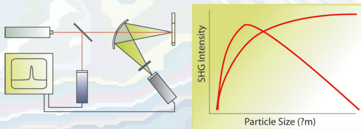
Second-Harmonic Generation
