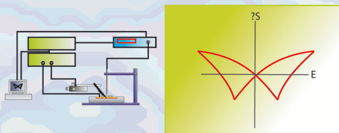
Piezoelectricity
