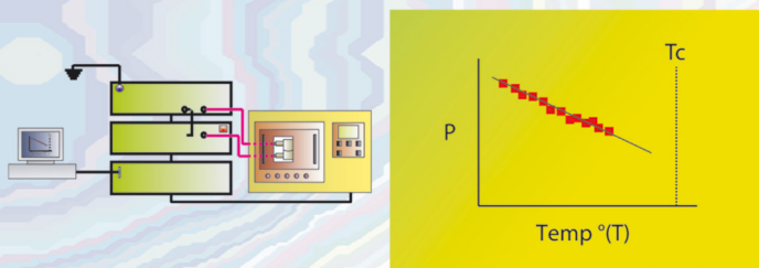
Pyroelectricity
