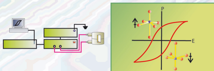
Ferroelectricity
